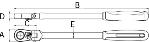
BOERMFLCG11 – 11mm Flex Head Cushion Grip Wrench
